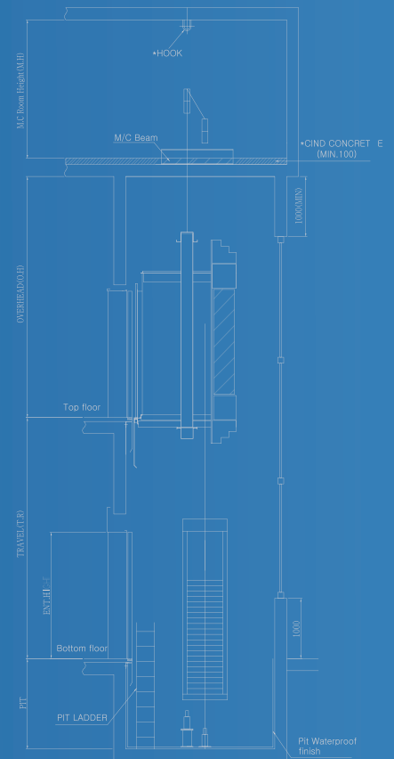
HOISTWAY SECTION
