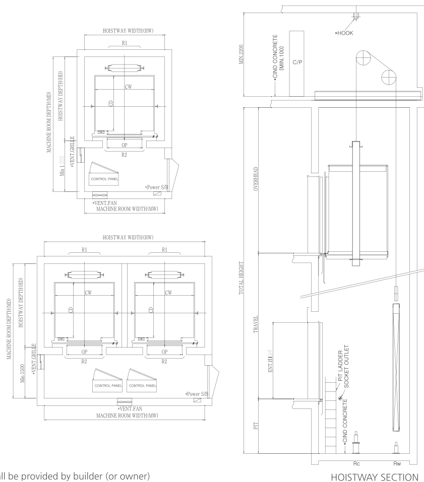
HOISTWAY SECTION
